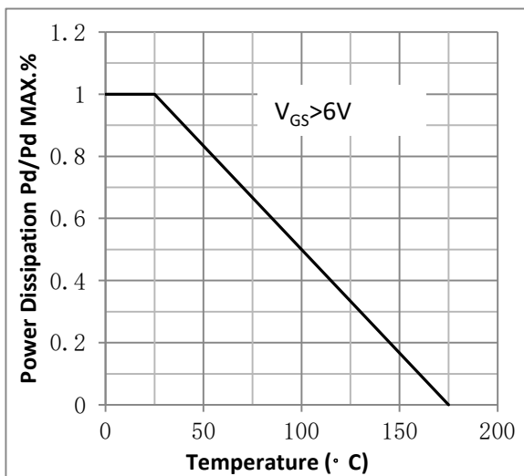
Fig.3 Power Dissipation
